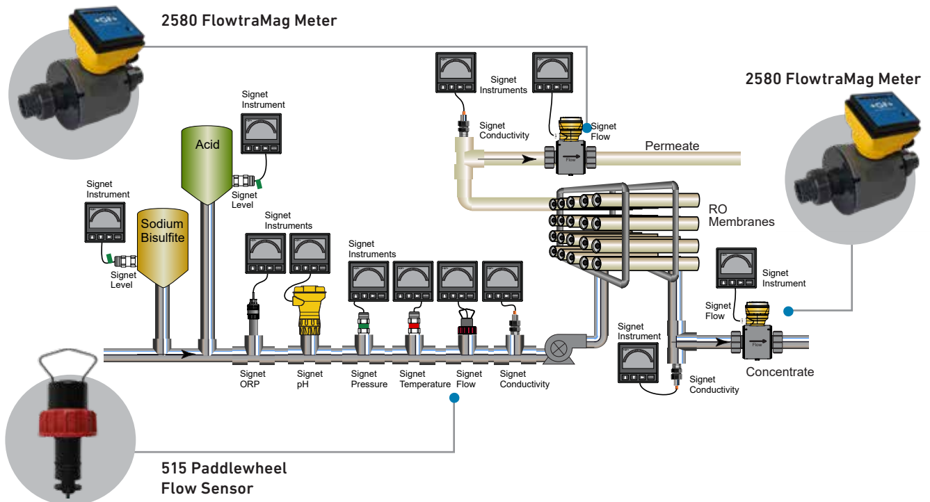
Example Application: Reverse Osmosis
