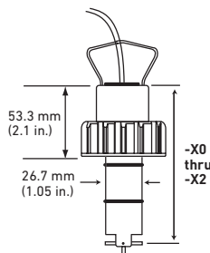
PVC Mount (0.5 to 4 in. pipe range only)
