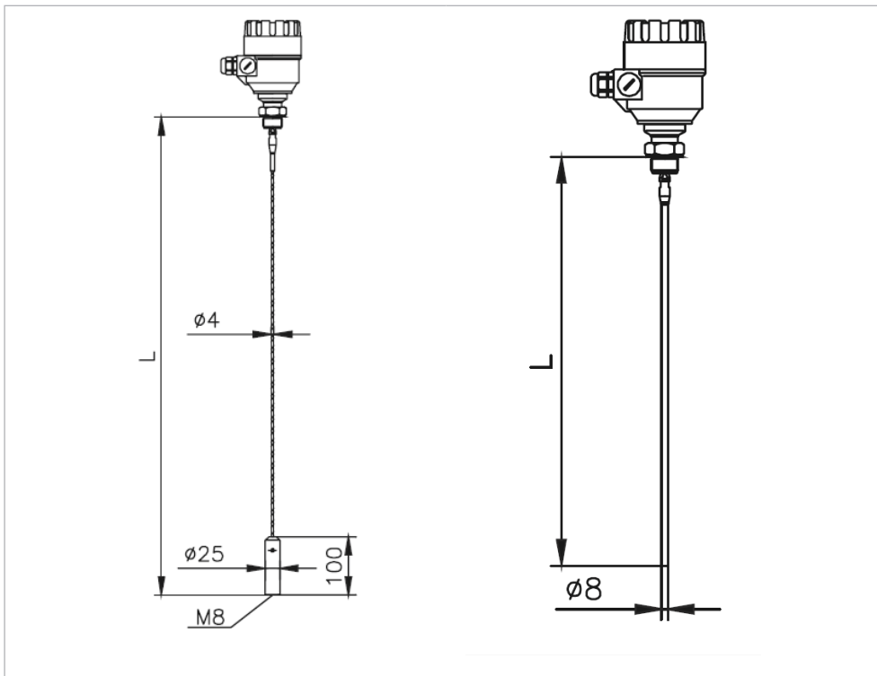
Type 2291 Cable Version L = 6 m (19.69 ft)
