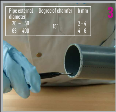
Deburr pipe ends with deburrer
