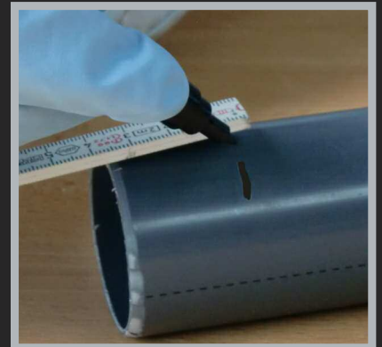
Marking of plug-in depth
