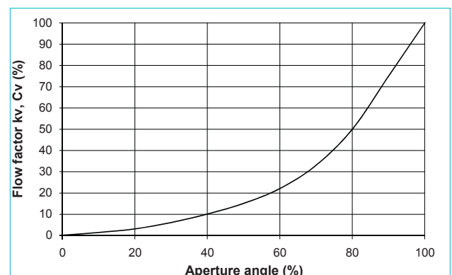
Flow characteristics of ELGEF Plus ball valve
