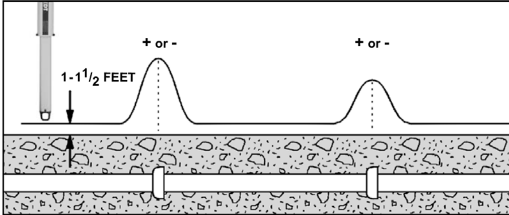
Figure 25: Signal Patterns Provided by Cast-Iron Pipes
